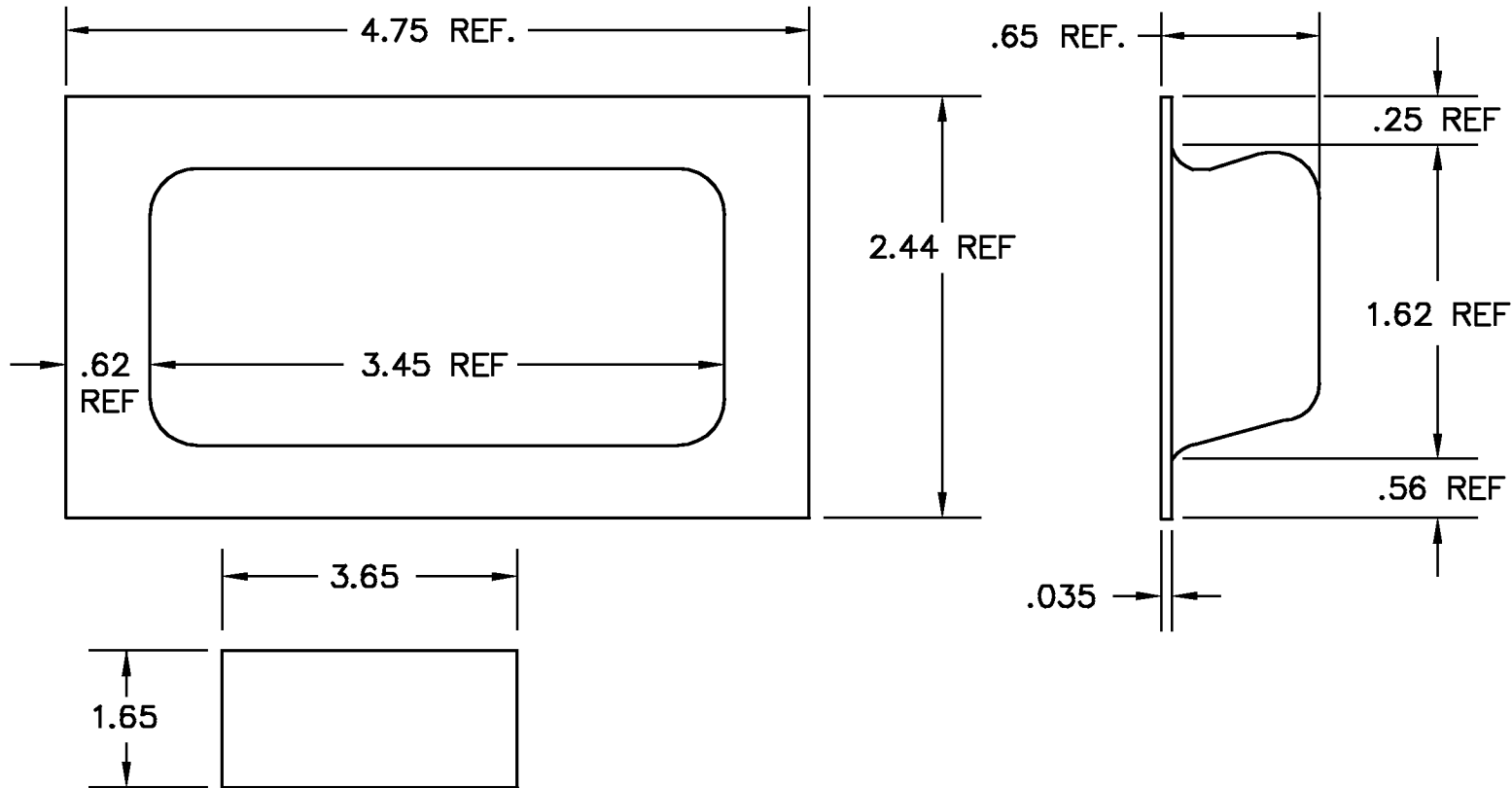
MOUNTING TEMPLATE
