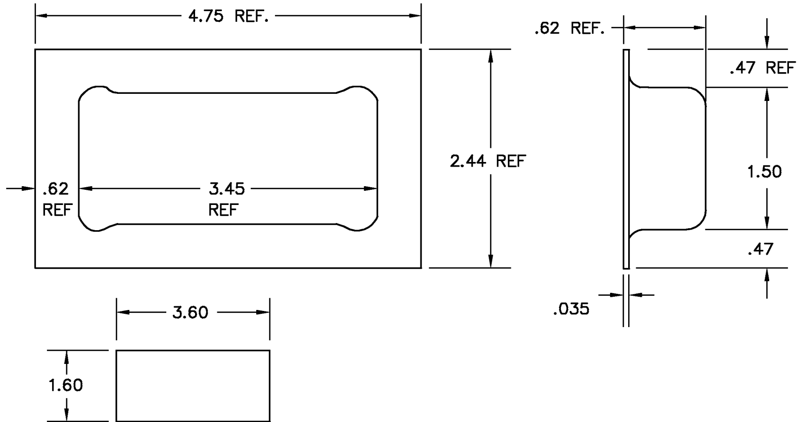
MOUNTING TEMPLATE
